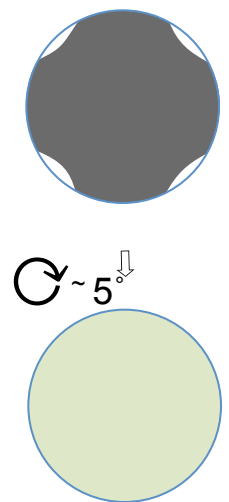
③ Optic Normal or "Flash Figure"
