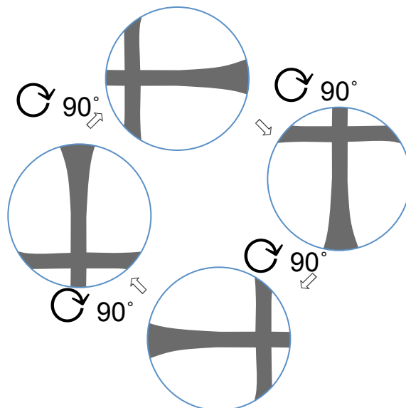
② Off-centered Uniaxial Optic Axis Figure
