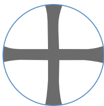
① Centered Uniaxial Optic Axis Figure
